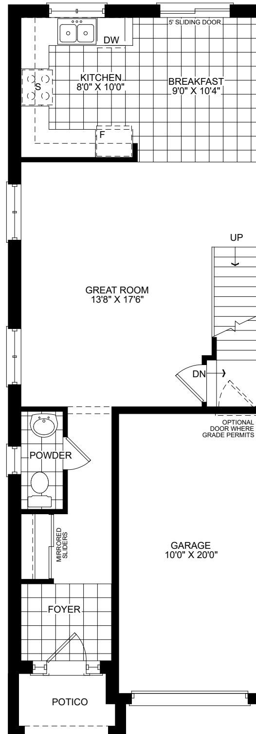
Ground Floor Elevation A
